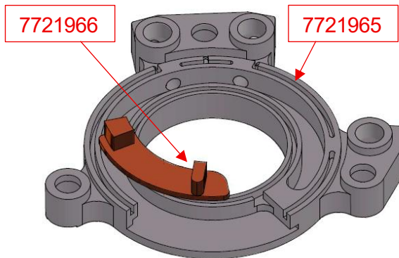
7721965 & 772966 Old Manifold/Adjustment Piece Combo
