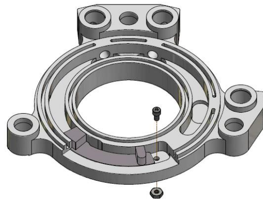
7723703 New Manifold/Adjustment Piece Combo
